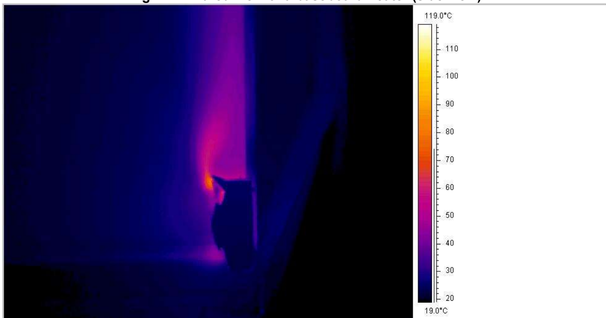
Fig. 1 – Infrared view of a baseboard heater (side view)
