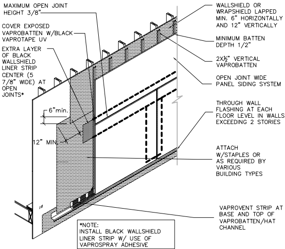
OPEN JOINT RAIN SCREEN-WIDE PANEL
