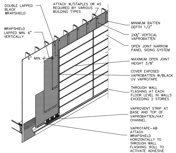
RAIN SCREEN OPEN JOINT -NARROW PANEL A.B.
