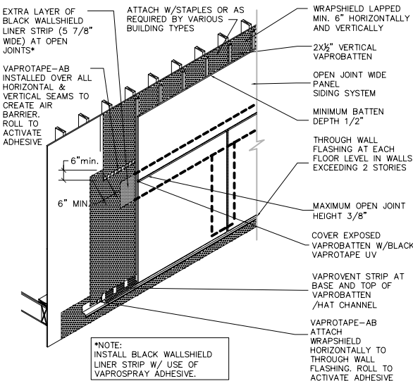
RAIN SCREEN OPEN JOINT-WIDE PANEL -A.B.
