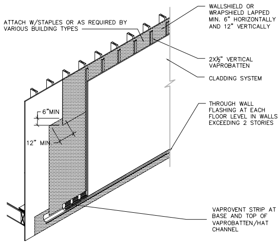
TYPICAL RAIN SCREEN
