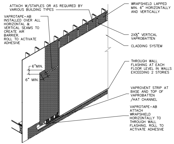
RAIN SCREEN-AIR BARRIER
