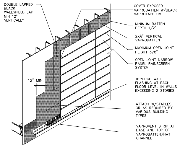
OPEN JOINT RAIN SCREEN-NARROW PANEL
